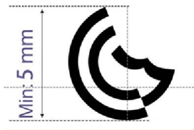
Fig. 3: GC Marking, minimum dimensions
